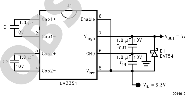
FIGURE 1. Step-Up Converter
